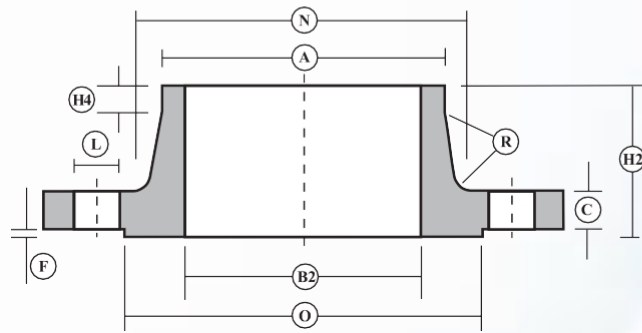
Steel Welding Neck Flange
