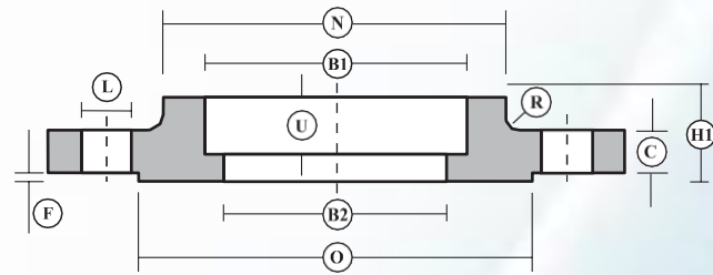
Socket Welding Flange
